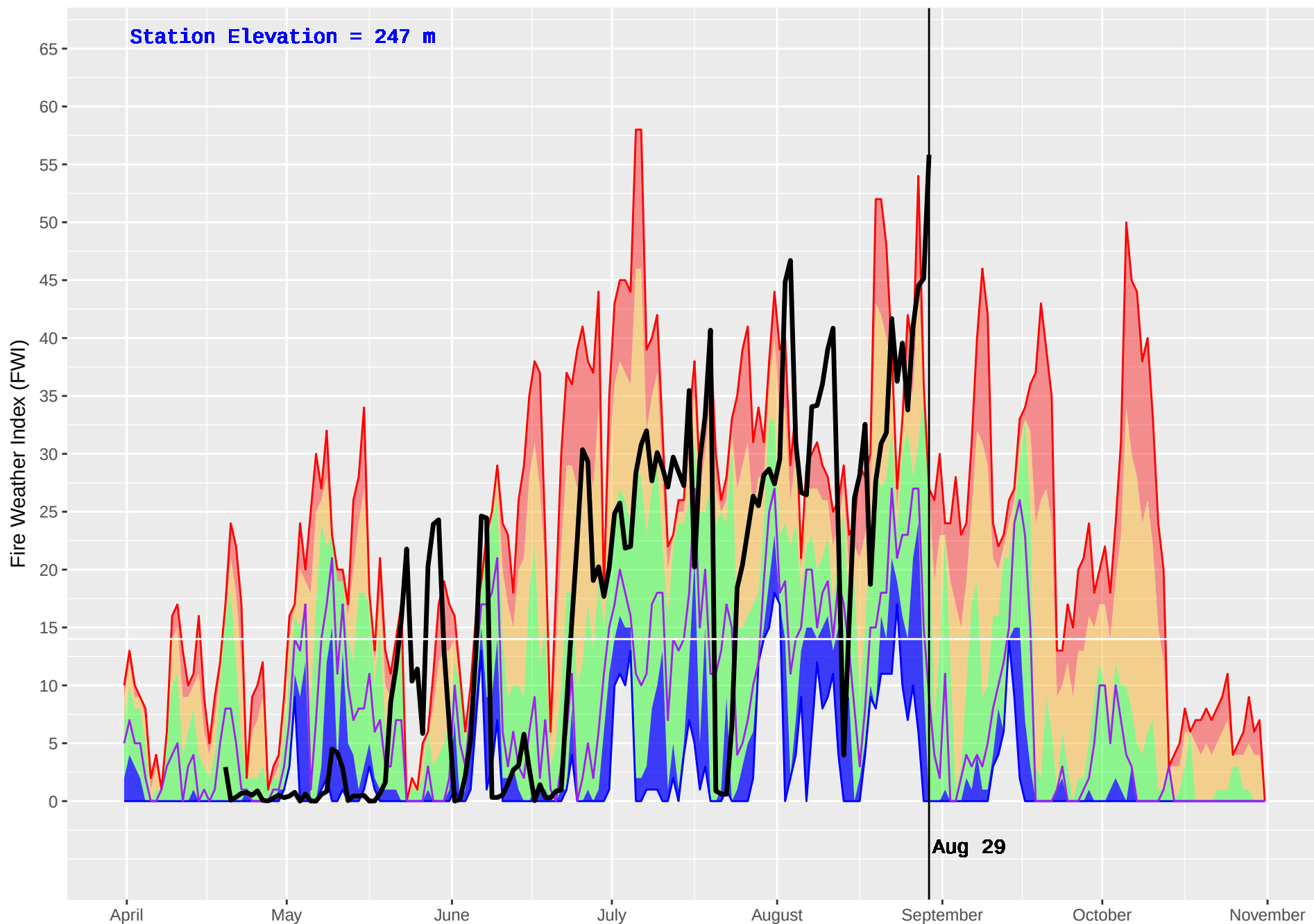
FORD MOUNTAIN (1144) : Historical (2012–2016) and Current (2017) Noon Fire Weather Index (FWI)
